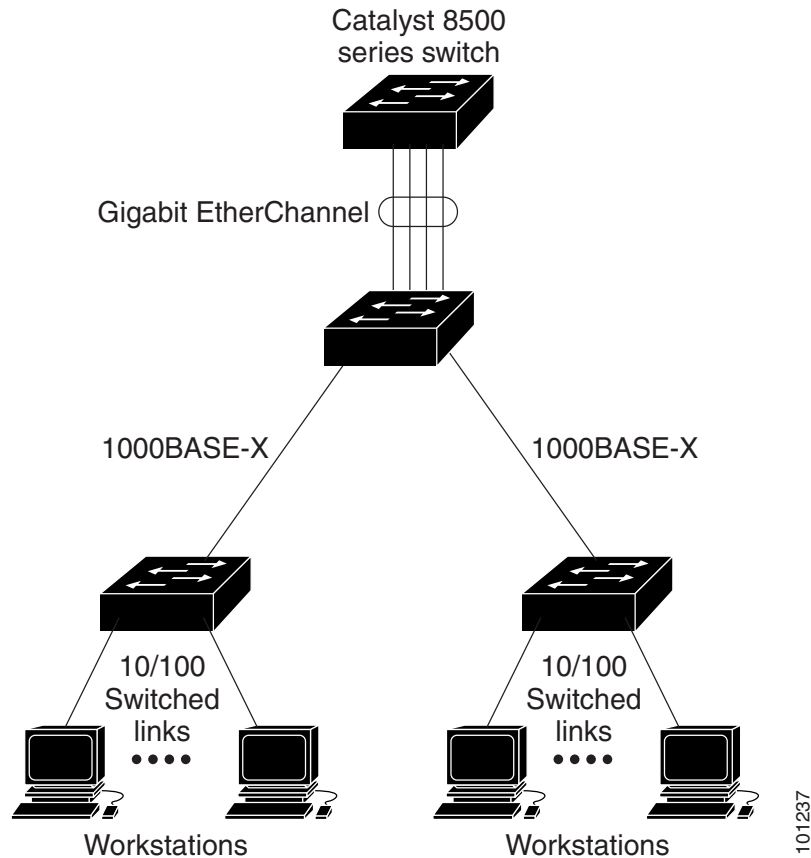
Figure 39-1 Typical EtherChannel Configuration
