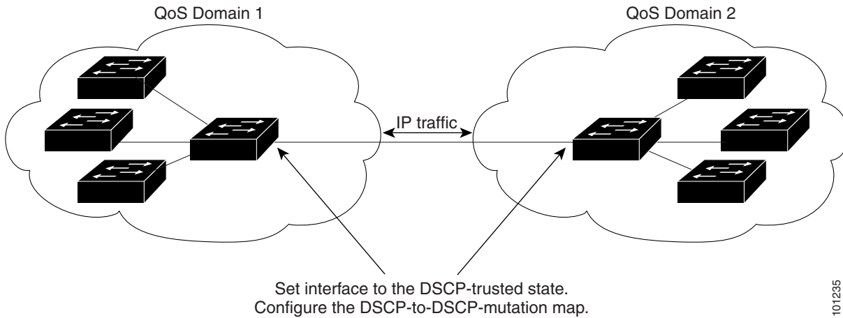
Figure 34-11 DSCP-Trusted State on a Port Bordering Another QoS Domain
