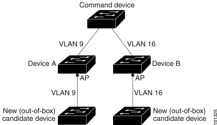
Figure 8-5 Discovery of Newly Installed Switches
