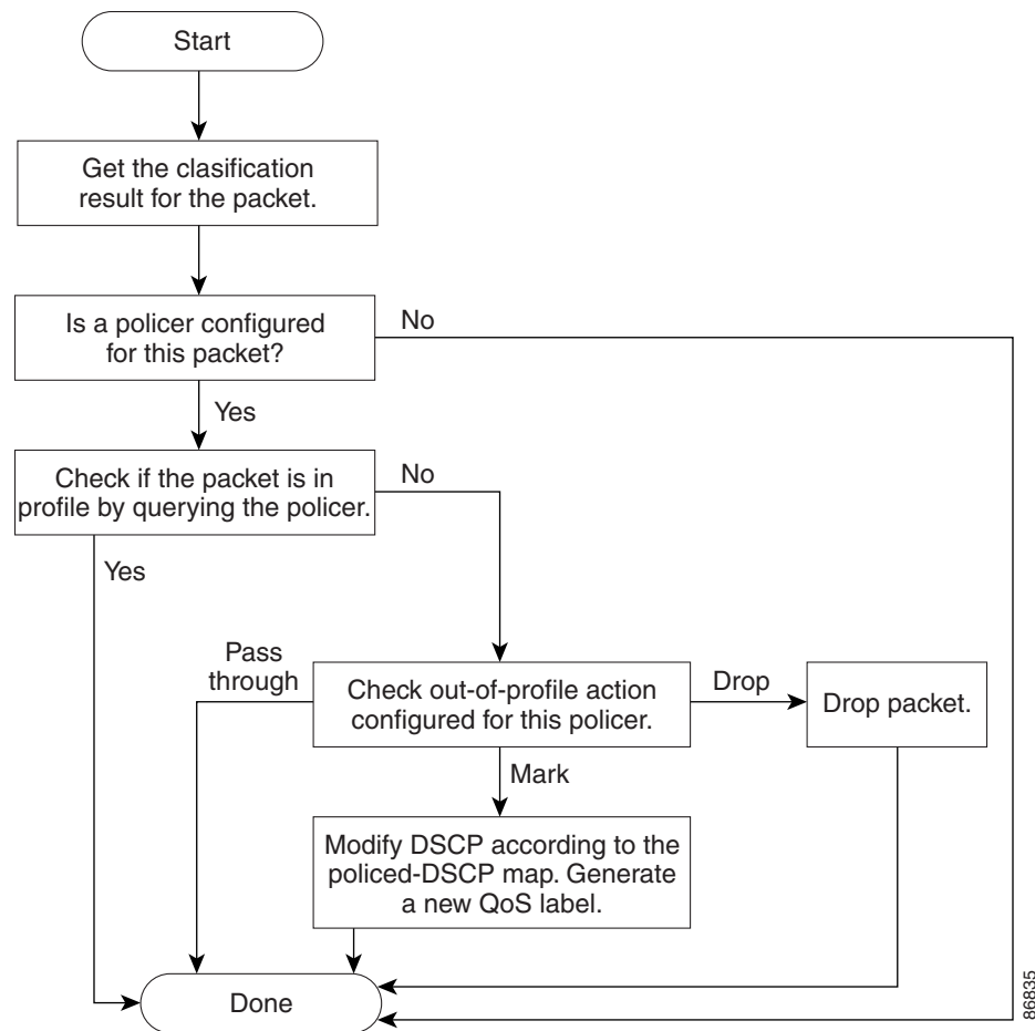
Figure 34-4 Policing and Marking Flowchart on Physical Ports
