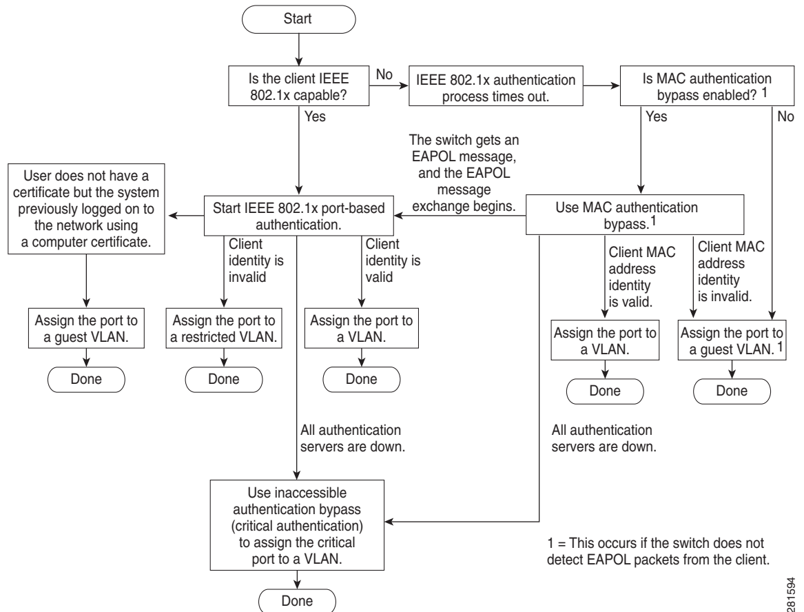
Figure 12-2 Authentication Flowchart
